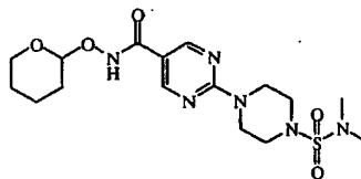
intermediate 9
